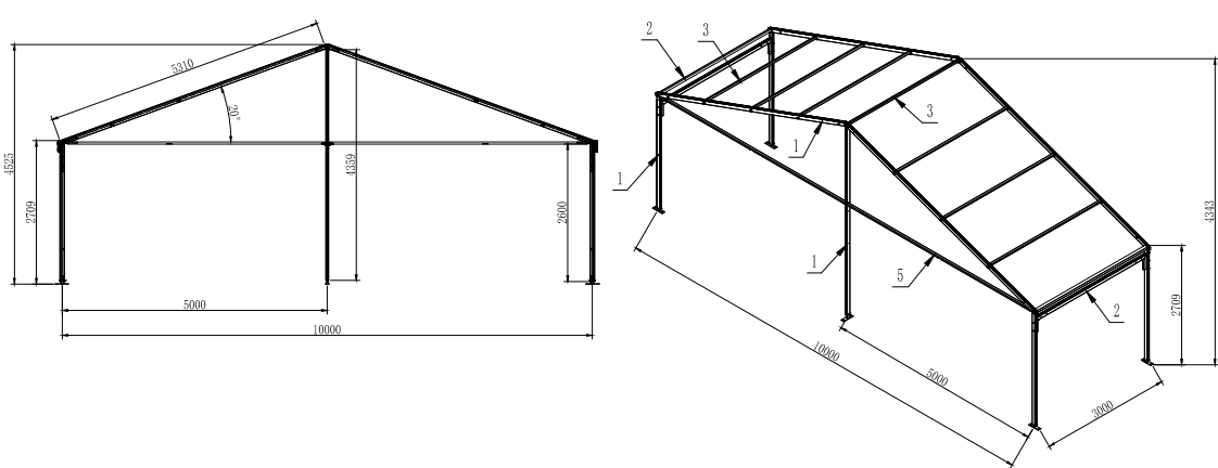
10m Span (3m Bay)
