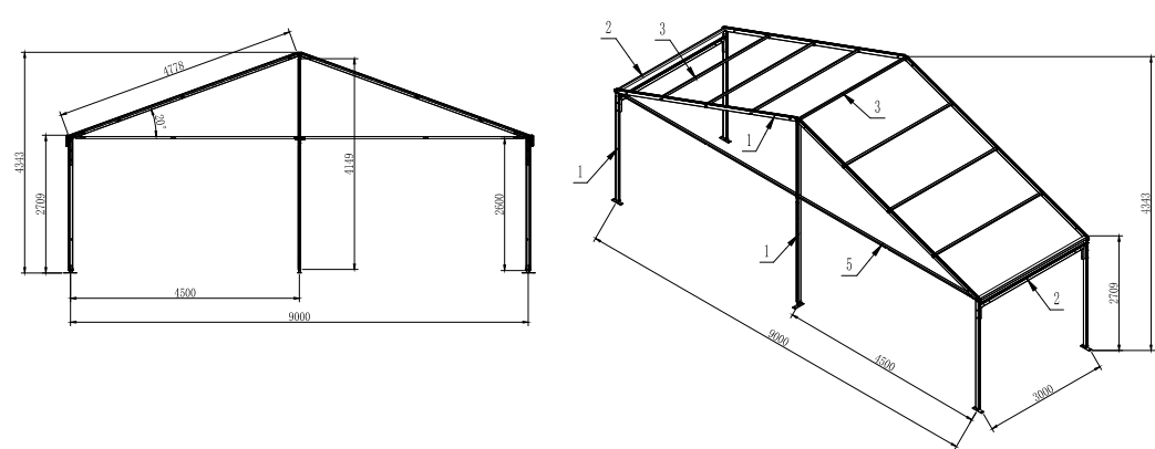
9m Span (3m Bay)
