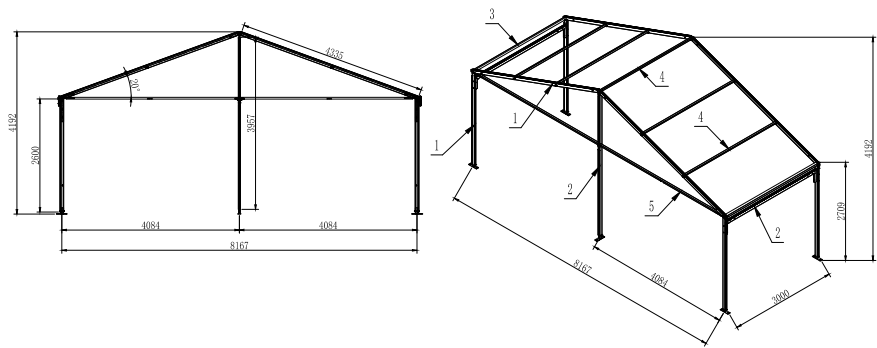
8m Span (3m Bay)
